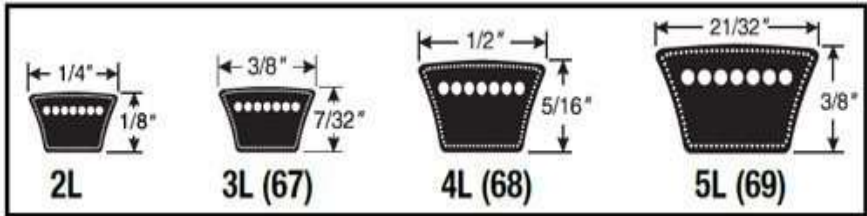
Fractional HP V-Belt Profiles
