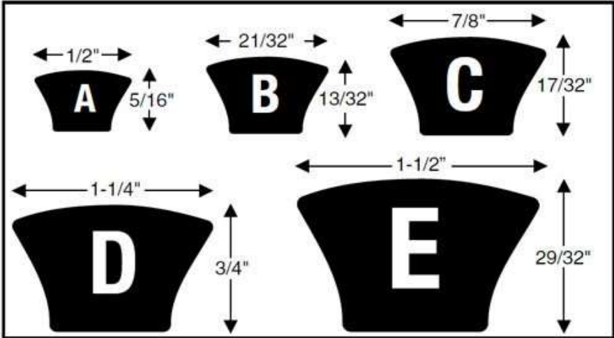
Classic V-Belt Profiles
