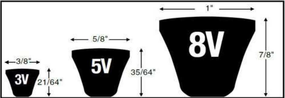
Narrow V-Belt Profiles
